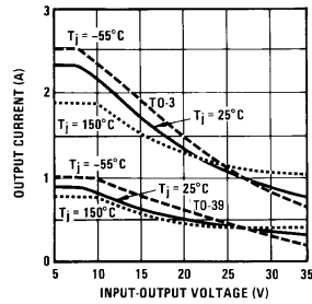
Current Limit Characteristics (Note 5)
